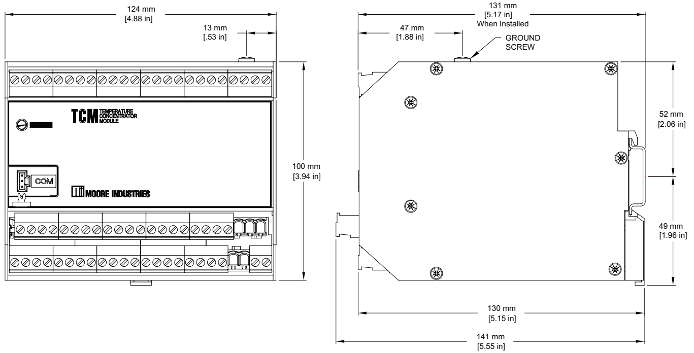
Figure 6. TCM Dimensions
